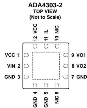
Figure 4. Pin Configuration
