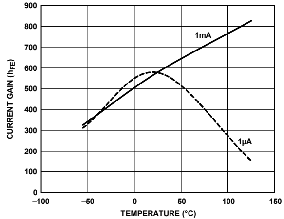
Figure 7. Current Gain vs. Temperature (Excludes I CB0 )
