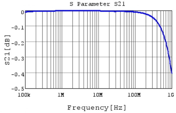
RDER71H474K1S1H03A S21 DC0V, 25degC
