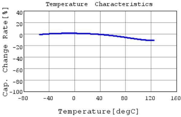
RDER71H474K1S1H03A C-Temp. capchange, DC0.0V
