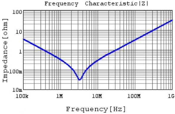
RDER71H474K1S1H03A |Z| DCOV, 25degC
