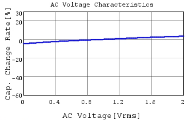
RDER71H474K1S1H03A C-AC Voltage capchange, I
