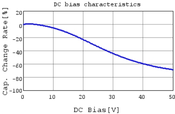
RDER71H474K1S1H03A C-DC bias capchange, 25.0
