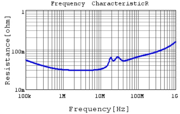
RDER71H474K1S1H03A R DCOV, 25degC
