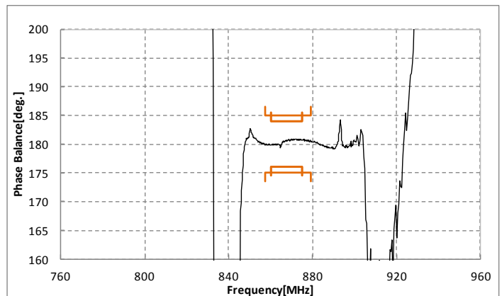
Phase balance
