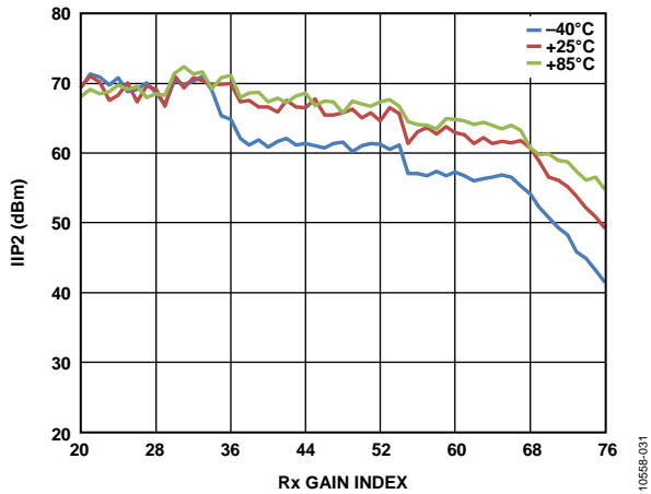
Figure 29. Second-Order Input Intercept Point (IIP2) vs. Rx Gain Index, f_1 = 60 MHz, f_2 = 61 MHz
