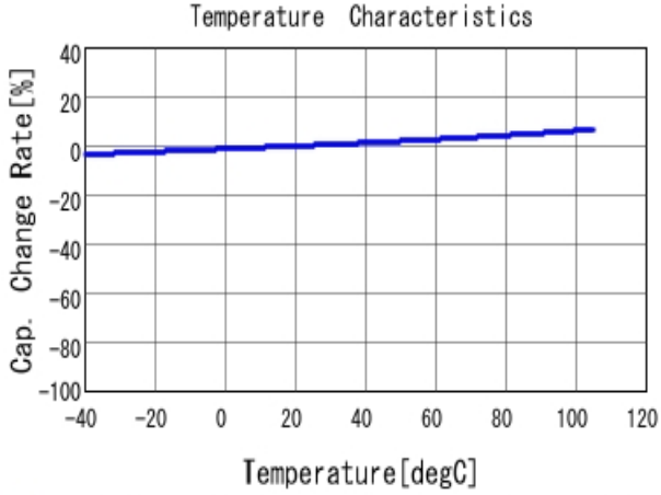
■ ECASD60E477M006K00 C-Temp. capchange, DCOV, AC1Vrms
