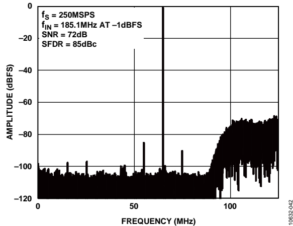
Figure 46. 33% Bandwidth Mode, Tuning Word = 5
