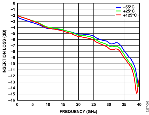
Figure 6. Insertion Loss vs. Frequency at Various Temperatures
