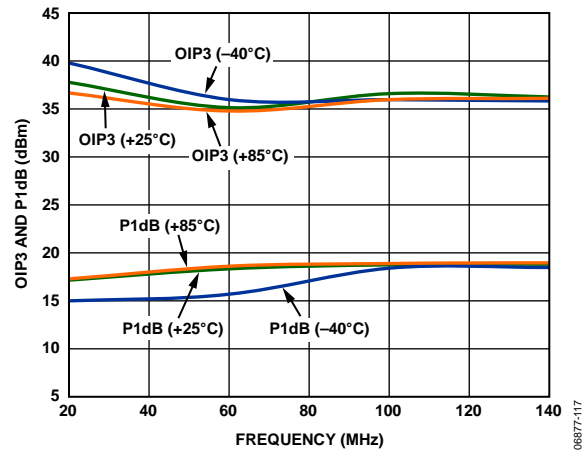
Figure 17. OIP3 and P1dB vs. Frequency and Temperature
