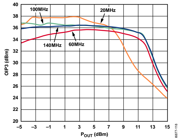
Figure 18. OIP3 vs. Output Power ( P_{out} ) and Frequency
