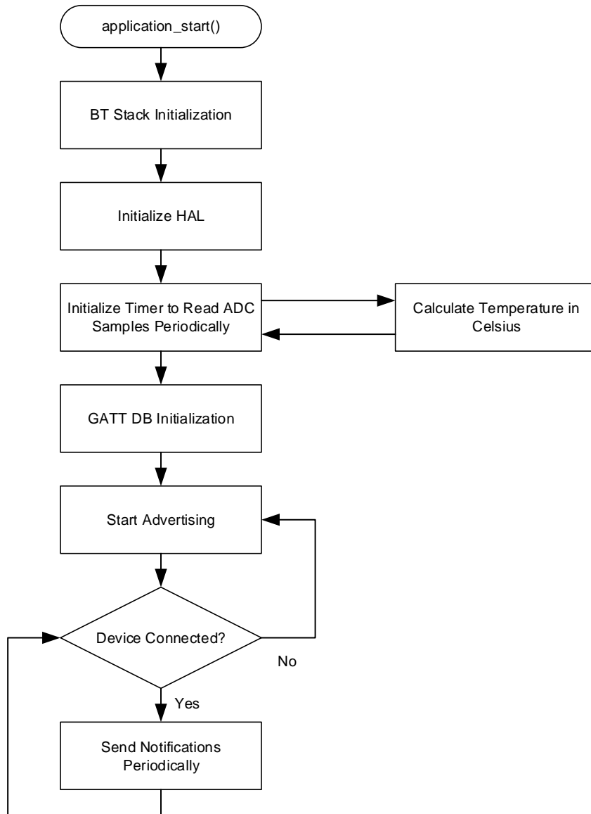
Figure 4-1. thermistor_app Flowchart
