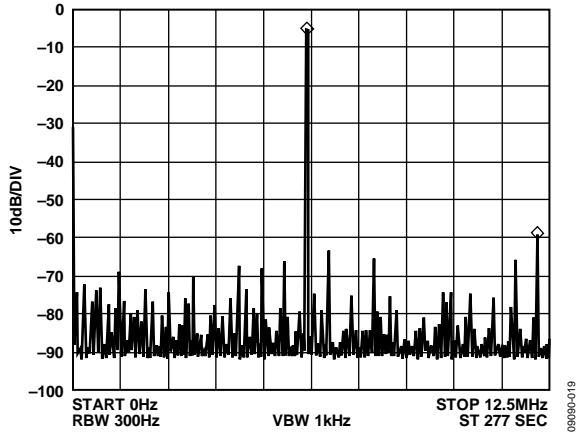
Figure 19. f_{CLK} = 25 \text{ MHz} , f_{OUT} = 6.1 \text{ MHz} , Frequency Word = 0x3E76C8B4
