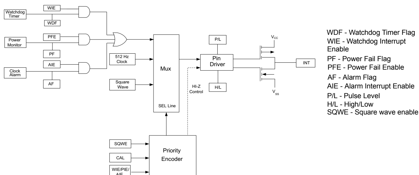
Figure 101. Interrupt Block Diagram
