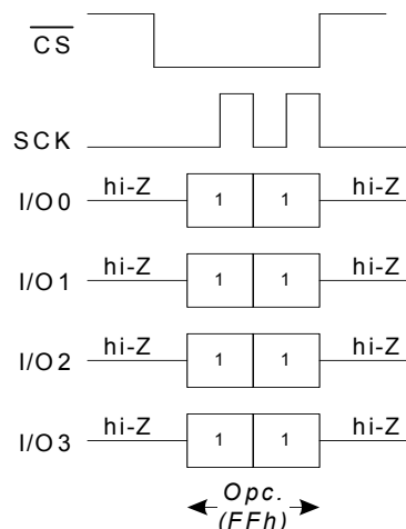
Figure 18. Enable SPI Instruction in QPI Mode
