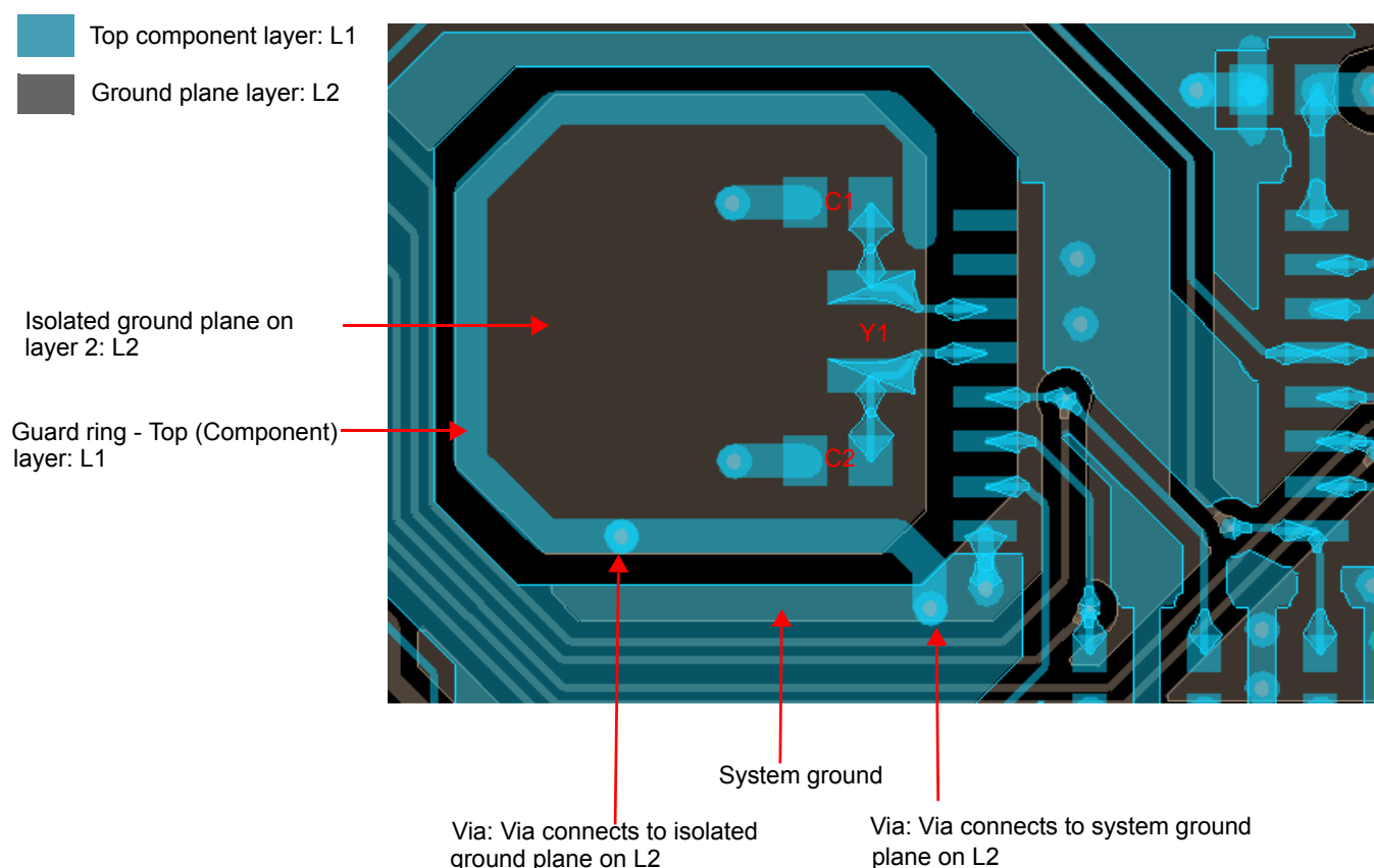
Figure 103. Recommended Layout for RTC
