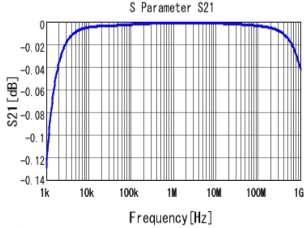
■ ECASD41C106M060K00 S21 DCOV, 25degC
