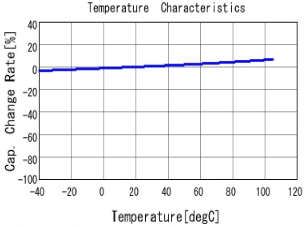
■ ECASD41C106M060K00 C-Temp. capchange, DCOV, AC1Vrms
