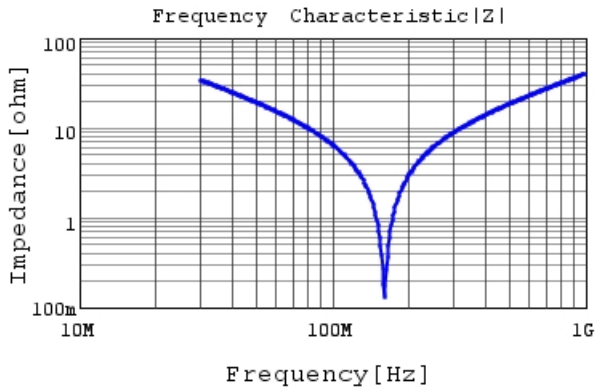
RDE5C2A151J0K1H03B |Z| DCOV, 25degC
