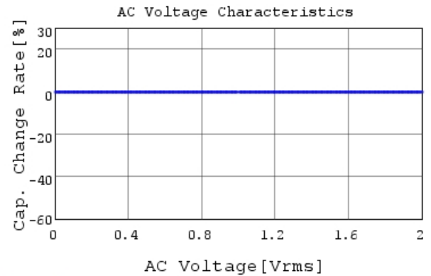
RDE5C2A151J0K1H03B C-AC Voltage capchange, 1
