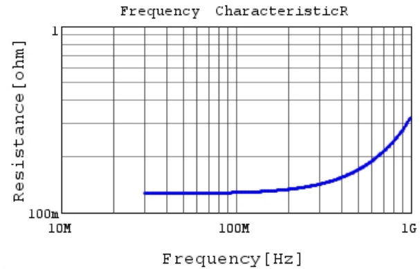
RDE5C2A151J0K1H03B R DCOV, 25degC
