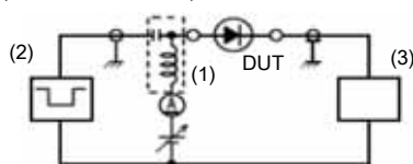
(Measurement circuit)
