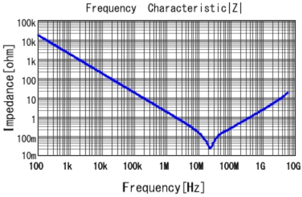
GRM188R71E104KA01 |Z| DCOV, 25degC
