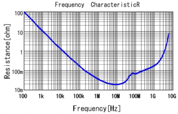
GRM188R71E104KA01 R DCOV, 25degC
