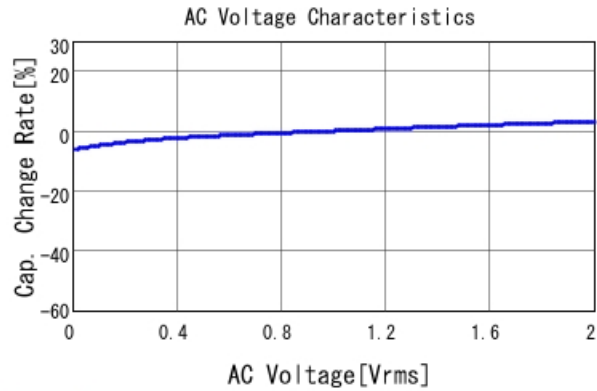
GRM188R71E104KA01 C-AC Voltage capchange, DCOV, 25
