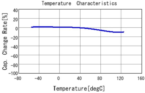
GRM188R71E104KA01 C-Temp. capchange, DC0.0V, AC1.C
