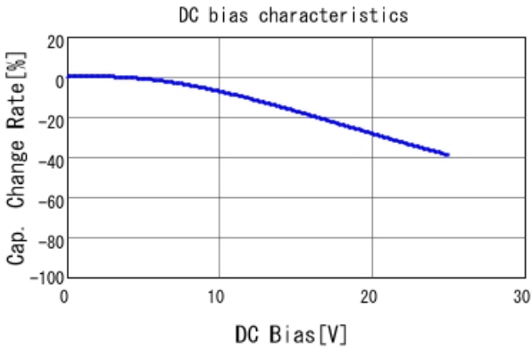
GRM188R71E104KA01 C-DC bias capchange, 25.0degC, A
