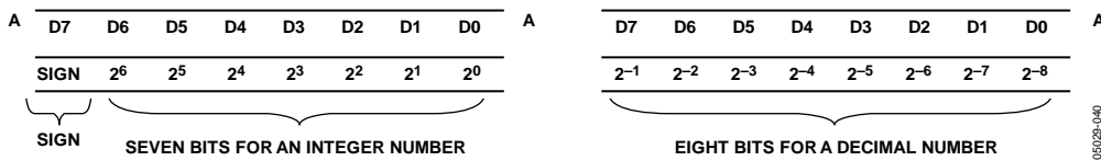
Figure 39. Format of Stored Tolerance in Sign Magnitude Format with Bit Position Descriptions (Unit is Percent; Only Data Bytes are Shown)
