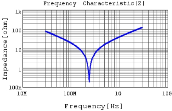
RDE5C2A680J0M1H03A |Z| DCOV, 25degC
