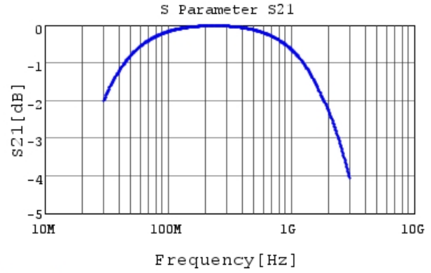
RDE5C2A680J0M1H03A S21 DCOV, 25degC
