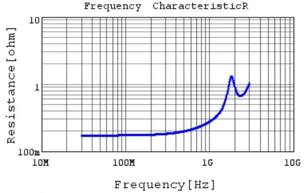
RDE5C2A680J0M1H03A R DCOV, 25degC
