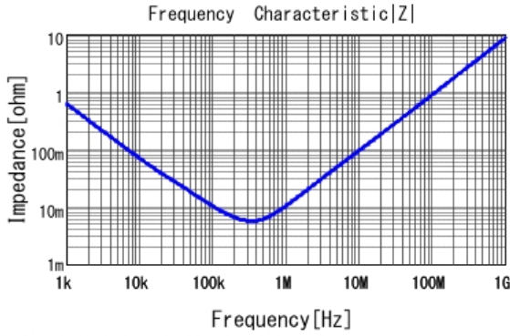
■ ECASD40D337Y009KA0 |Z| DCOV, 25degC
