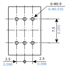
Recommended PC board
