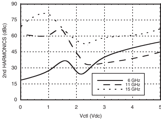
Second Harmonics vs. Control Voltage, Pin = -10 dBm
