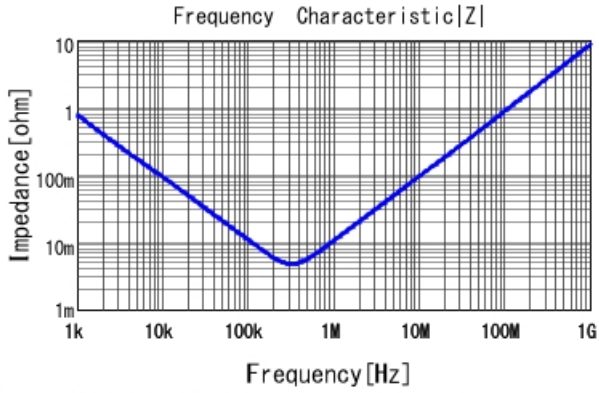
ECASD40D227M009K00 |Z| DC0V, 25degC
