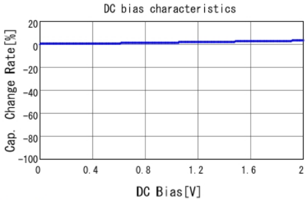
ECASD40D227M009K00 C-DC bias capchange, 25.0degC,
