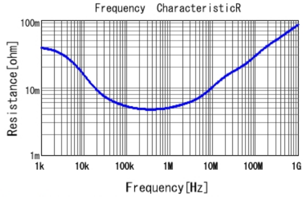
ECASD40D227M009K00 R DC0V, 25degC
