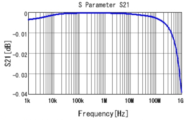
ECASD40D227M009K00 S21 DCOV, 25degC
