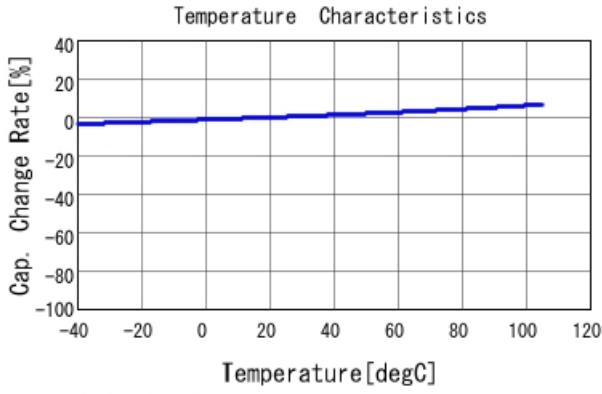
ECASD40D227M009K00 C-Temp. capchange, DCOV, AC1Vrr
