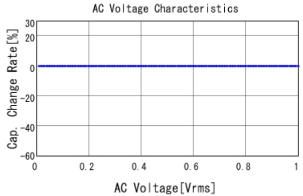
ECASD40D227M009K00 C-AC Voltage capchange, DC0V, 2
