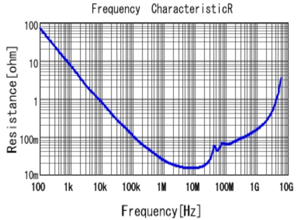
■ GRM188R72A104KA35 R DCOV, 25degC
