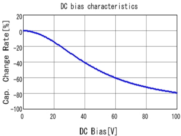
■ GRM188R72A104KA35 C-DC bias capchange, 25.0degC, AC1.
