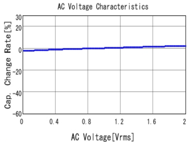
■ GRM188R72A104KA35 C-AC Voltage capchange, DCOV, 25.0d
