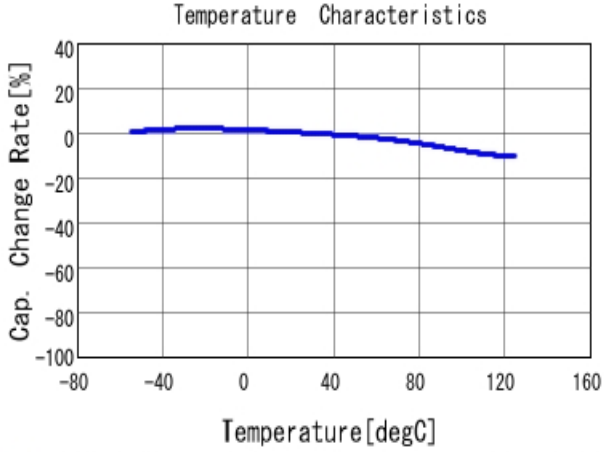
■ GRM188R72A104KA35 C-Temp. capchange, DC0.0V, AC1.0V r m
