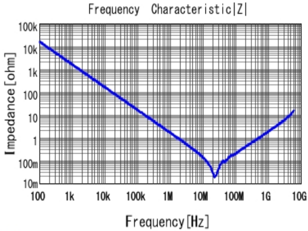
■ GRM188R72A104KA35 |Z| DCOV, 25degC
