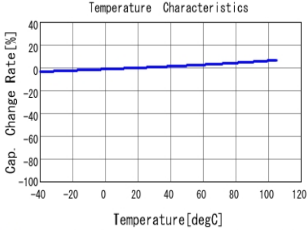
■ ECASD41E226M040KA0 C-Temp. capchange, DCOV, AC1Vrms
