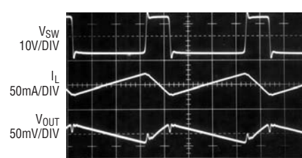
Switching Waveforms (LT3465A)
