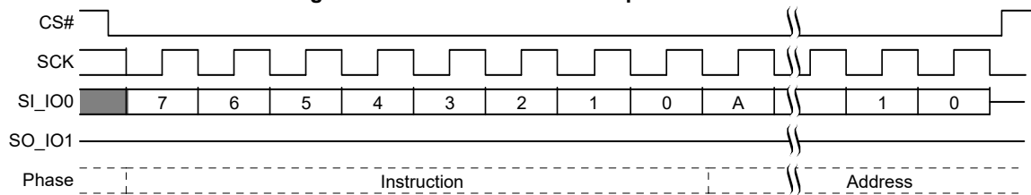
Figure 105. SPRP Command Sequence [60, 61]
