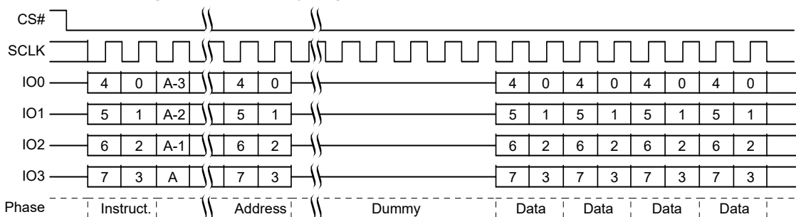
Figure 60. Read Any Register, QPI Mode, Command Sequence [30]
