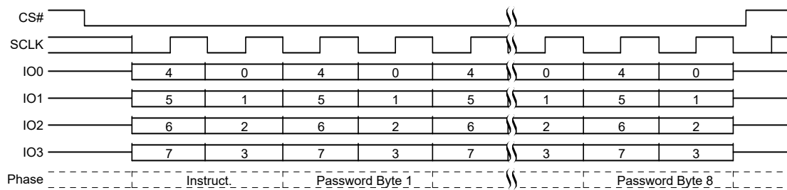
Figure 120. Password Unlock (PASSU) Command Sequence QPI mode
