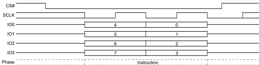
Figure 48. Clear Status Register (CLSR) QPI Mode
