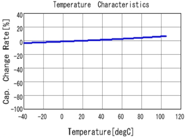
■ ECASD31C476M040KA0 C-Temp. capchange, DCOV, AC1Vrms
