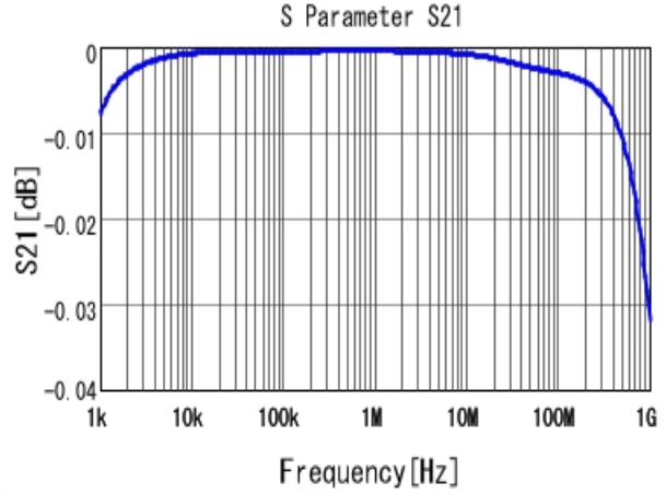
■ ECASD31C476M040KA0 S21 DCOV, 25degC
