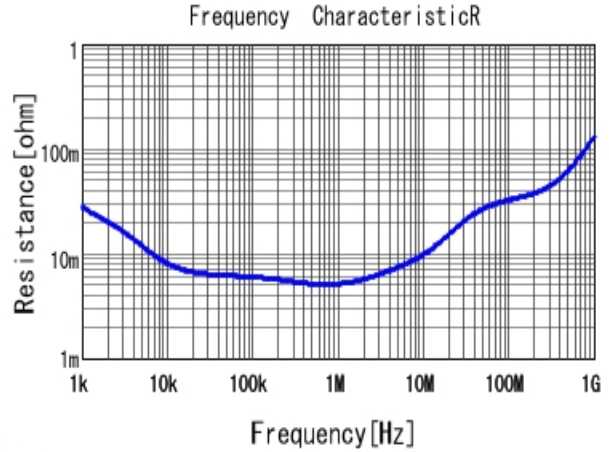
■ ECASD31C476M040KA0 R DCOV, 25degC
