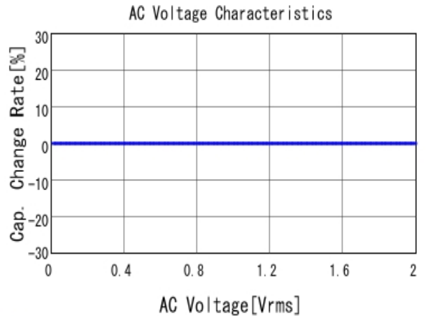
■ ECASD31C476M040KA0 C-AC Voltage capchange, DCOV, 25.0
