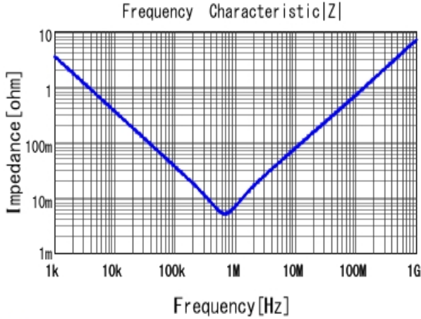
■ ECASD31C476M040KA0 |Z| DCOV, 25degC
