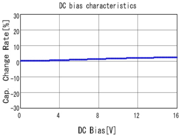
■ ECASD31C476M040KA0 C-DC bias capchange, 25.0degC, AC1
