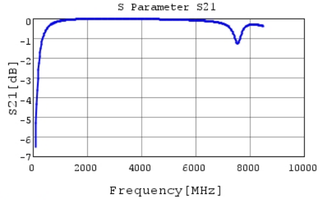
GCQ1555C1H8R5WB01 S21 DCOV, 25degC
