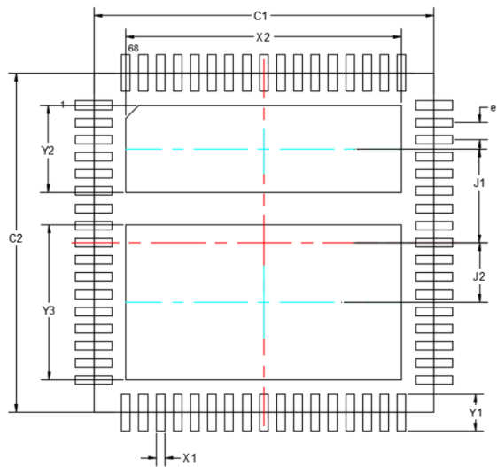
Figure 7.2. 68-Pin QFN Land Pattern
