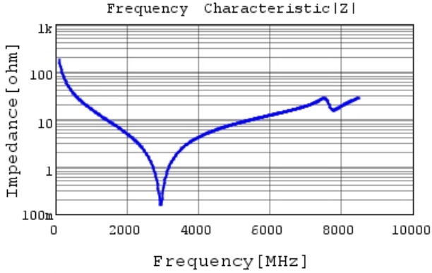
GCQ1555C1H8R8DB01 |Z| DC0V, 25degC
