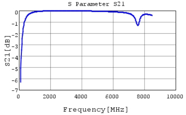
GCQ1555C1H8R8DB01 S21 DCOV, 25degC
