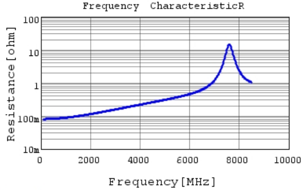
GCQ1555C1H8R8DB01 R DC0V, 25degC
