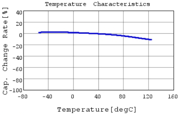
RCEC72A475MWK1H03B C-Temp. capchange, DC0.0V
