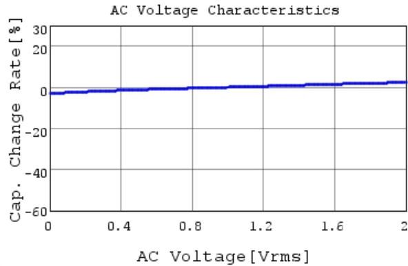
RCEC72A475MWK1H03B C-AC Voltage capchange, I
