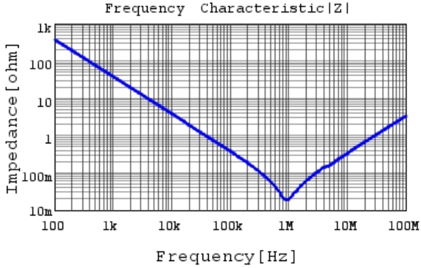
RCEC72A475MWK1H03B |Z| DC0V, 25degC
