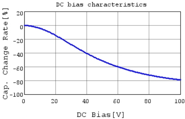
RCEC72A475MWK1H03B C-DC bias capchange, 25.0
