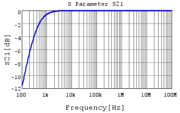
RCEC72A475MWK1H03B S21 DC0V, 25degC
