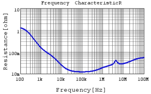
RCEC72A475MWK1H03B R DC0V, 25degC
