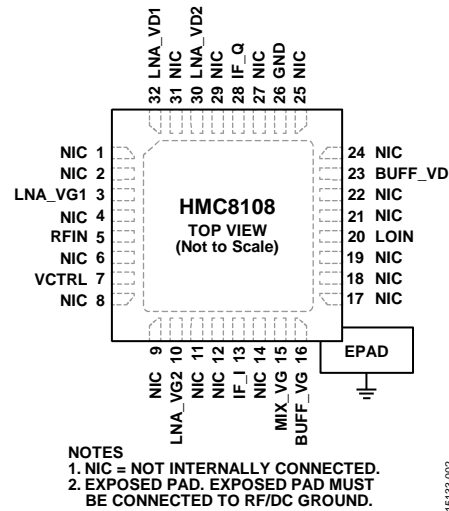
Figure 2. Pin Configuration
