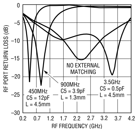
(4b) Series Shunt Matching
