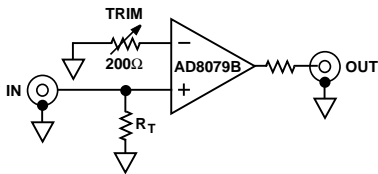
Optional Gain Trim (G = +2 → +2.2)
