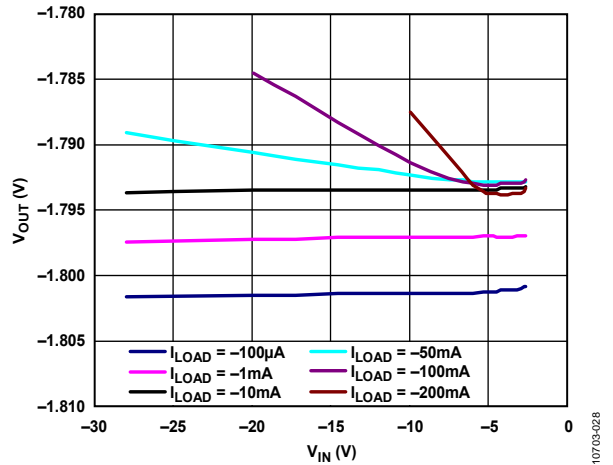
Figure 30. Output Voltage ( V_{OUT} ) vs. Input Voltage ( V_{IN} ), V_{OUT} = -1.8 V
