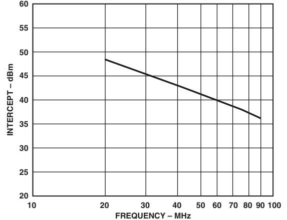
TPC 21. AD9631 Third Order Intercept vs. Frequency
