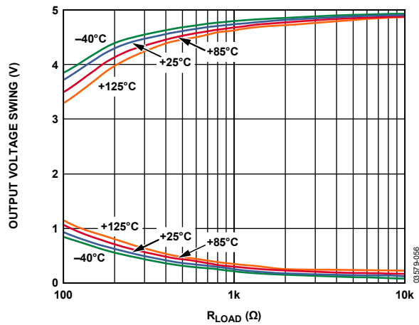
Figure 35. Output Voltage Swing vs. Load Resistance V_S = +5 V , V_{REF} = 2.5 V
