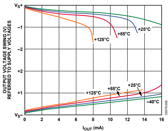
Figure 37. Output Voltage Swing vs. Output Current, V_S = 5 V , V_{REF} = 2.5 V
