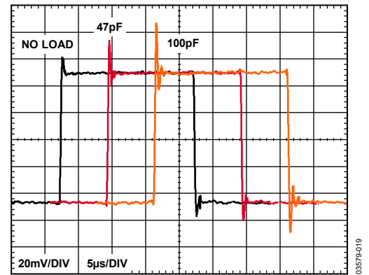
Figure 39. Small Signal Pulse Response for Various Capacitive Loads, V_S = 5 V , V_{REF} = 2.5 V
