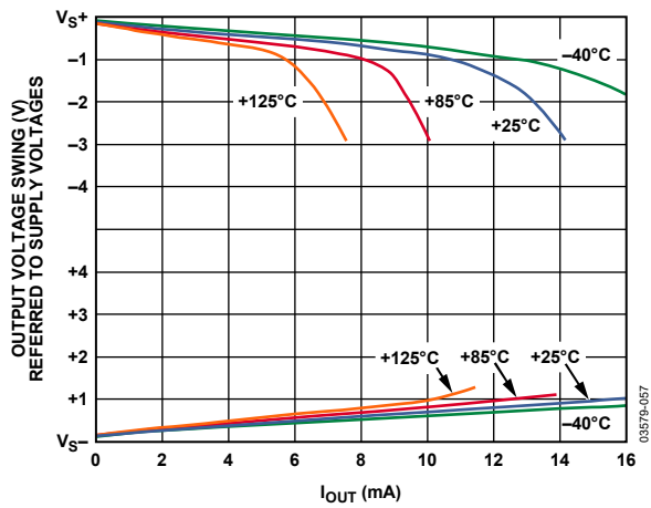
Figure 36. Output Voltage Swing vs. Output Current, V_S = \pm 15 V , V_{REF} = 0 V
