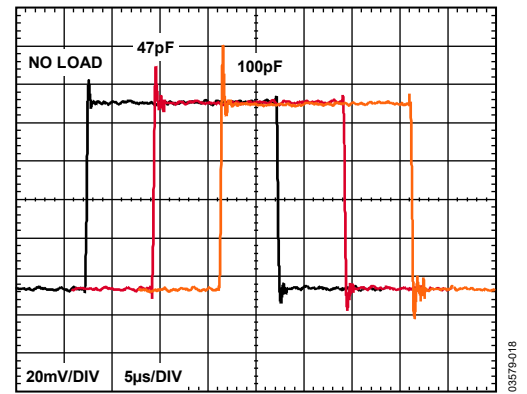
Figure 38. Small Signal Pulse Response for Various Capacitive Loads, V_S = \pm 15 V , V_{REF} = 0 V
