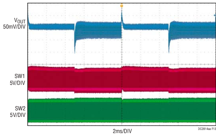
Figure 13. DC2814A-A Load Transients at 7.5V IN (Buck-Boost), 8V OUT , 0.3A to 2.7A Load Current
