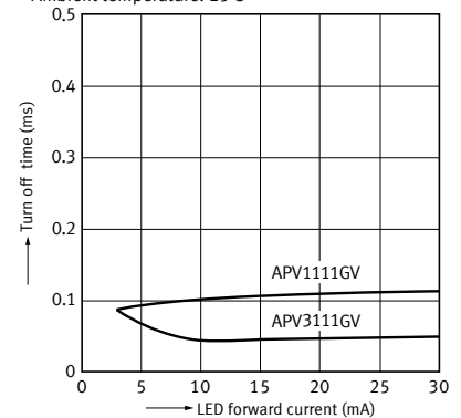
7. Turn off time vs. LED forward current characteristics
