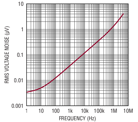
Integrated Voltage Noise (0.1Hz to Frequency Indicated)
