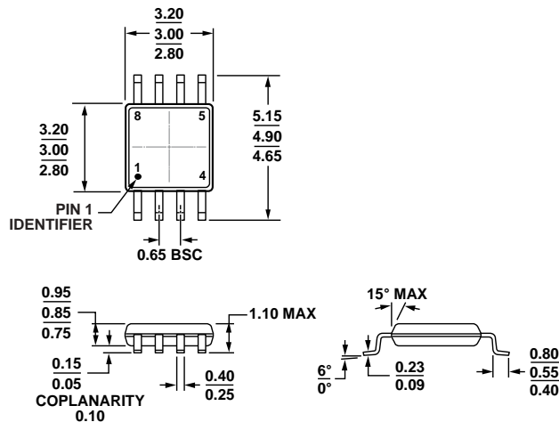
COMPLIANT TO JEDEC STANDARDS MO-187-AA Figure 51. 8-Lead Mini Small Outline Package [MSOP] (RM-8) Dimensions shown in millimeters
