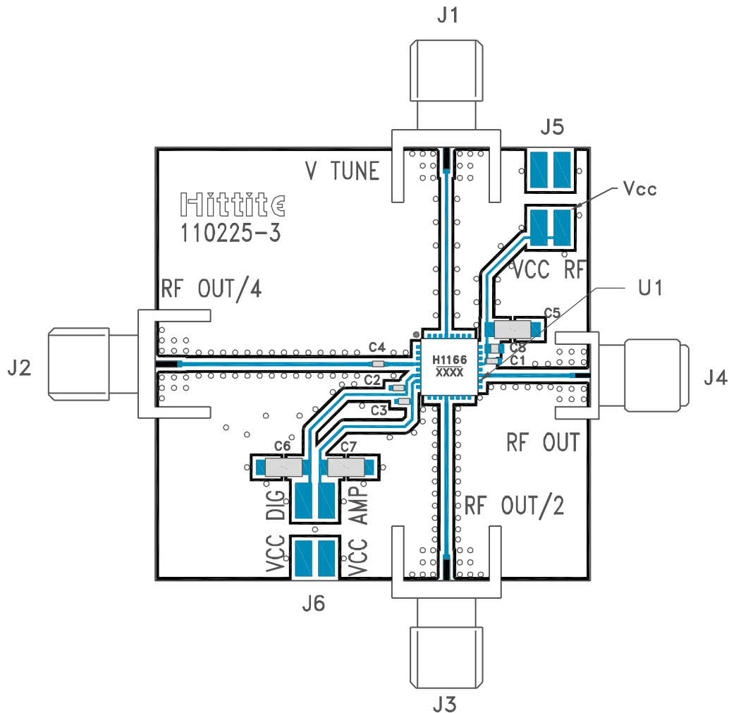
Figure 17. Evaluation PCB
