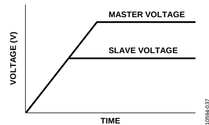
Figure 31. Coincident Tracking
