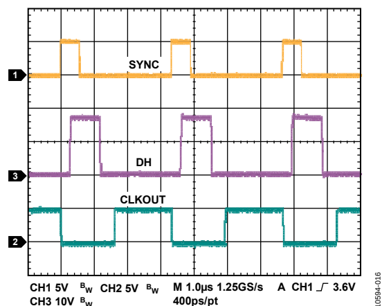
Figure 10. Synchronization and CLKOUT, f_{SYNC} = 300 kHz
