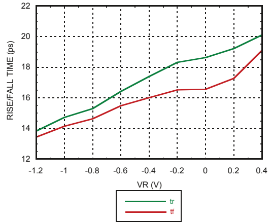
Rise / Fall Time vs. VR [2][3]
