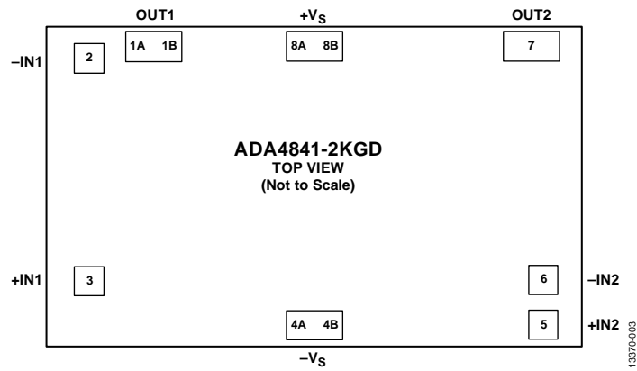
Figure 3. Pin Configuration
