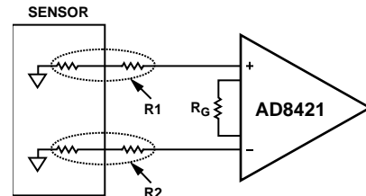
Figure 70. Source Resistance from Sensor and Protection Resistors
