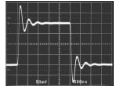
Small-Signal Transient ( A_V = -1, C_L = 1000\text{pF} )
