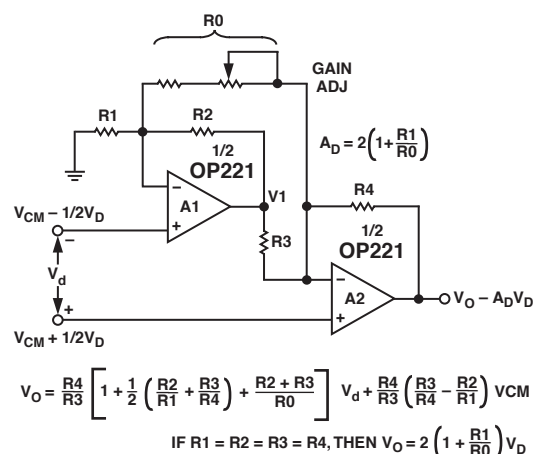
Figure 7. Two-Op Amp Circuit
