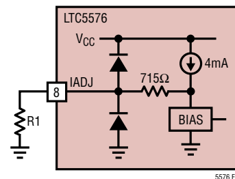
Figure 10. Current Adjust Pin Interface
