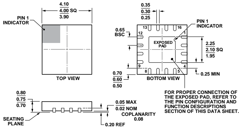
Figure 53. 16-Lead Lead Frame Chip Scale Package [LFCSP_WQ] 4 mm × 4 mm Body, Very Thin Quad (CP-16-23) Dimensions shown in millimeters
