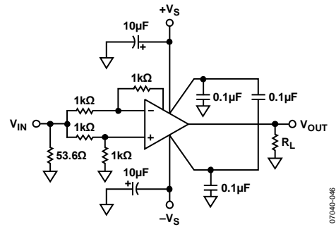
Figure 45. Common-Mode Rejection
